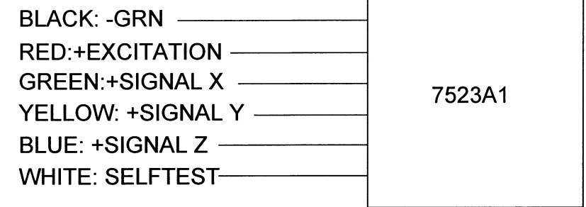
WIRING DIAGRAM
